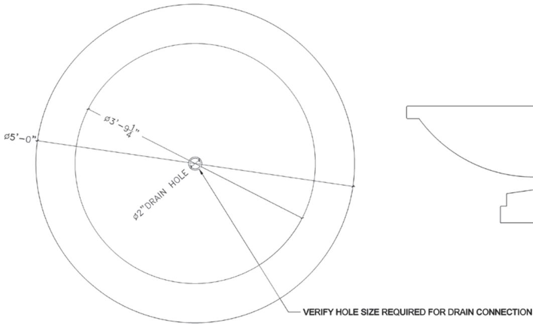
① PLAN VIEW - 5'Ø x 22"H MODIFIED CAPRI SCALE: 3" = 1'-0" REF: 3/L5.32
