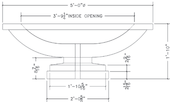
② ELEVATION VIEW - 5'Ø x 22"H MODIFIED CAPRI SCALE: 3" = 1'-0" REF: 3/L5.32
